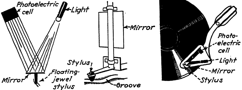
Photoelectric phonograph pickup.
